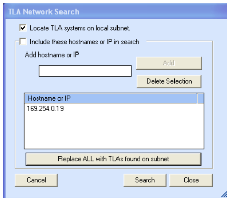
Figure 3-13: TLA Network Search dialog box
